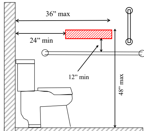
Dispenser Location Above Grab Bar
