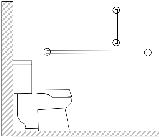
Side Wall Grab Bar for Water Closet
