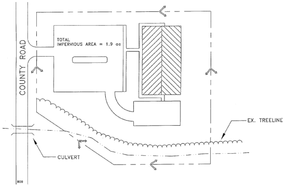
FIGURE 4-24 Sand Filter Example Site Plan Source: GSMM (2001)
