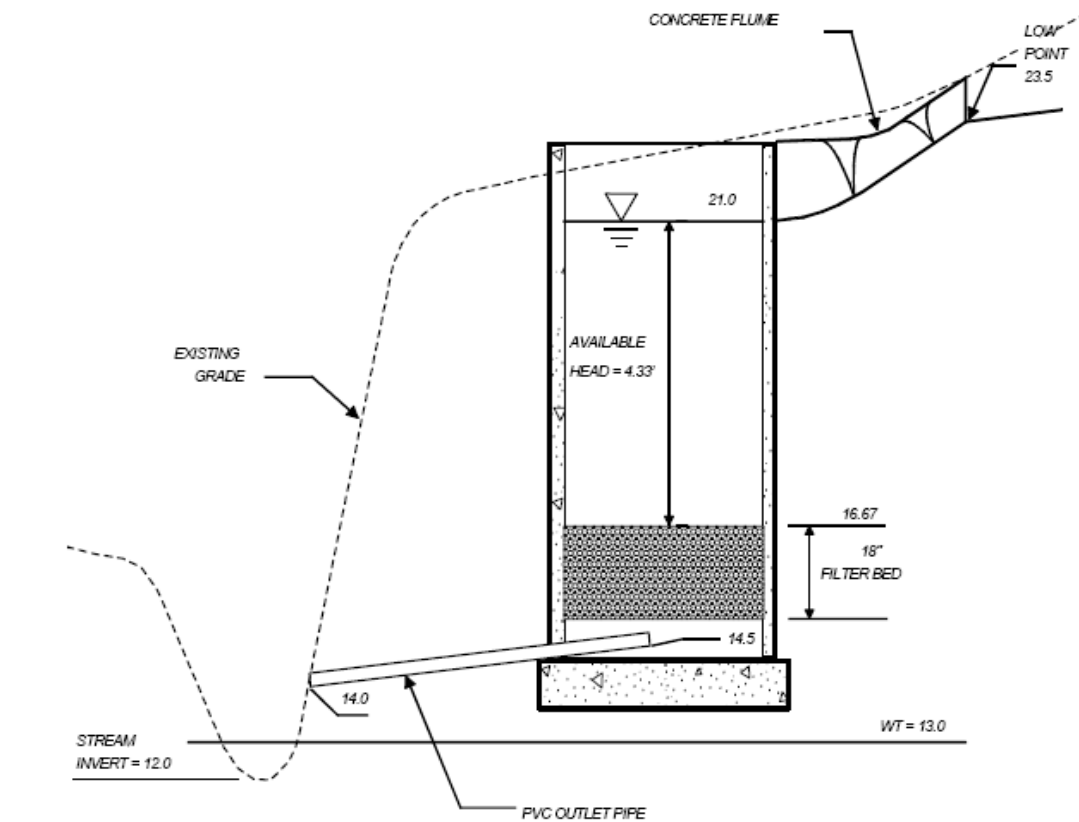
FIGURE 4-25 Head Diagram Source: GSMM (2001)
