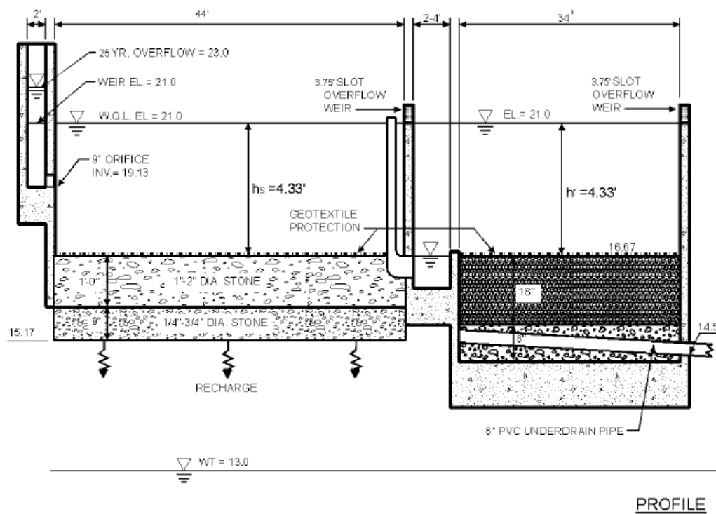
FIGURE 4-27 Sand Filter Site Plan View and Profile Source: GSMM (2001)
