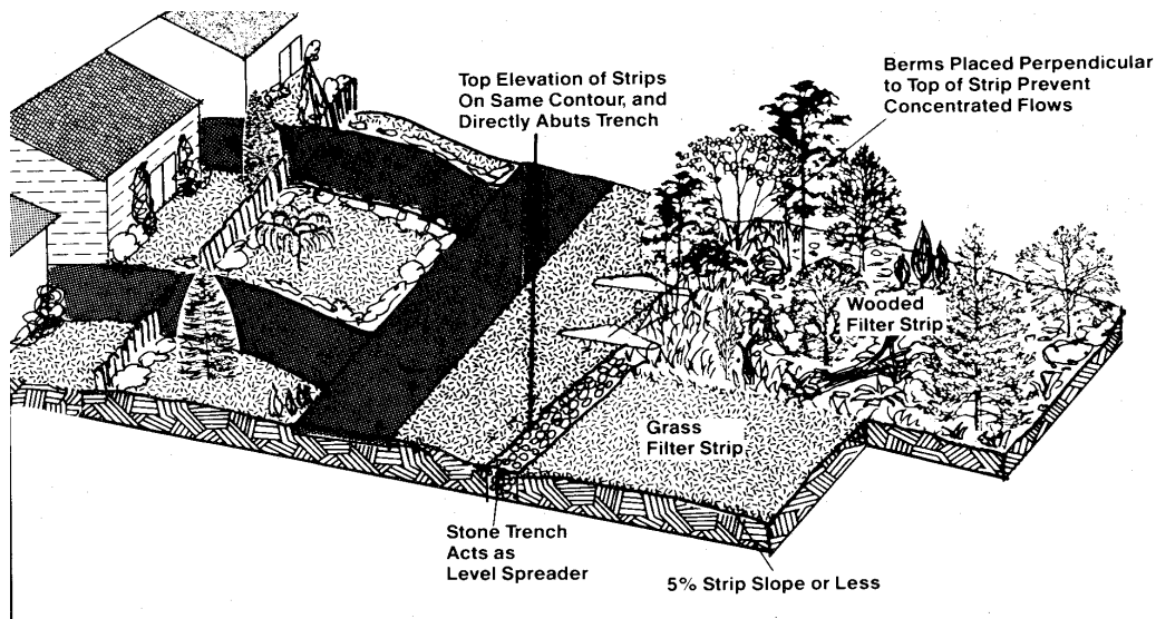
FIGURE 4-28 Filter Strip in Residential Area Adapted from Schueler (1987)
