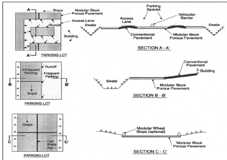
Figure 3.3.8-2 Modular Porous Paver System Section
