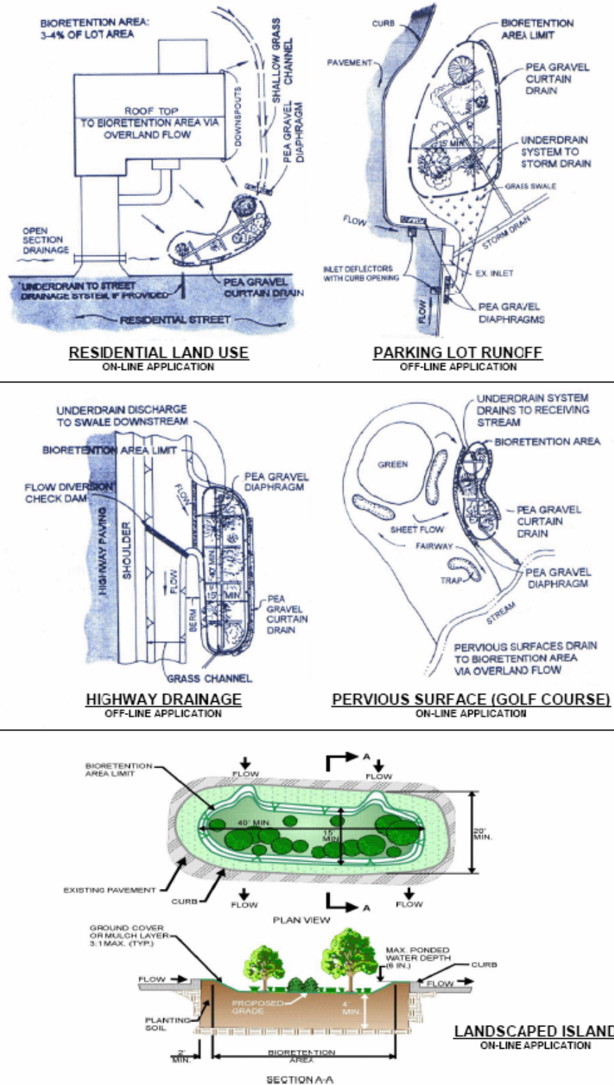
FIGURE 4-4 Bioretention Applications Source: GSMM (2001)
