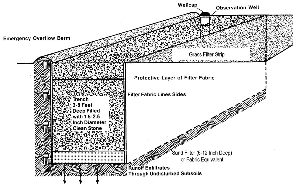
FIGURE 4-10 Typical Infiltration Trench Adapted from (1992); Source: GSMM (2001)
